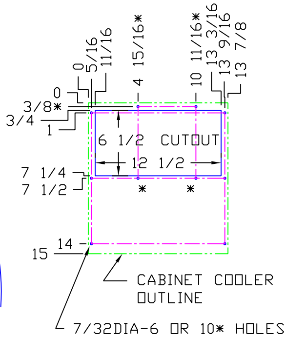
ENCLOSURE HOLE PATTERN
